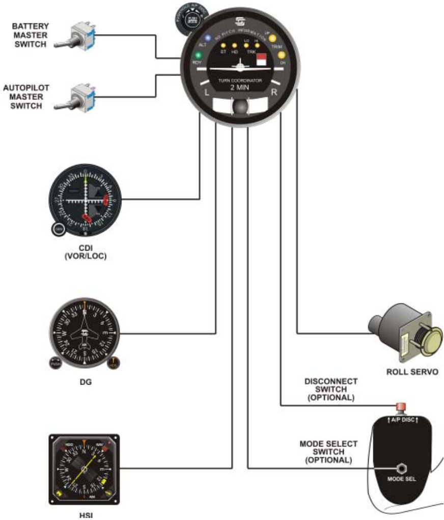
Fig. 1-1. System Twenty Block Diagram
